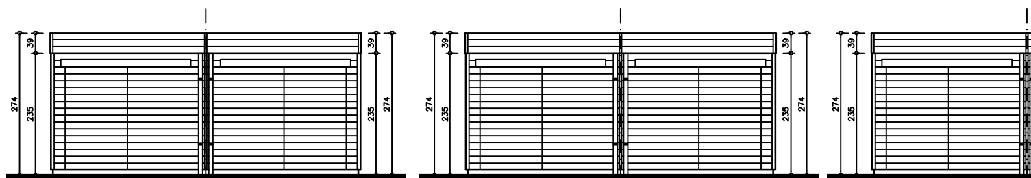
CARPORT + TUINBERGING Woning 6
