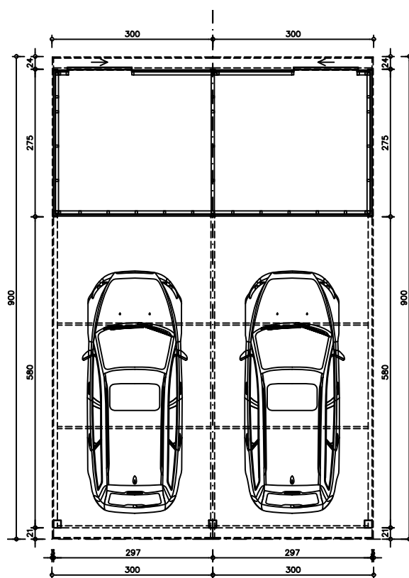
CARPORT + TUINBERGING Woning 5
