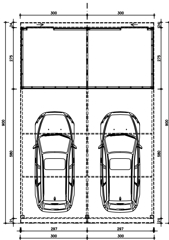
CARPORT + TUINBERGING Woning 3
