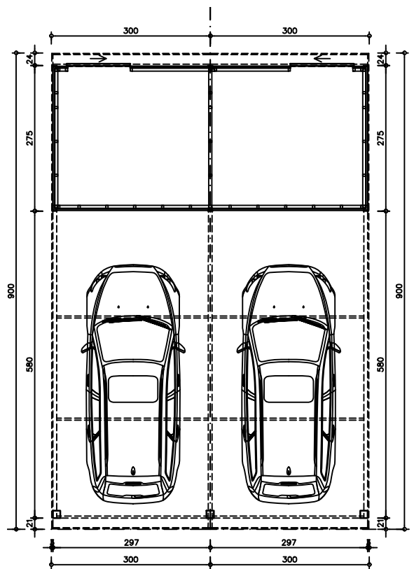
CARPORT + TUINBERGING Woning 5
