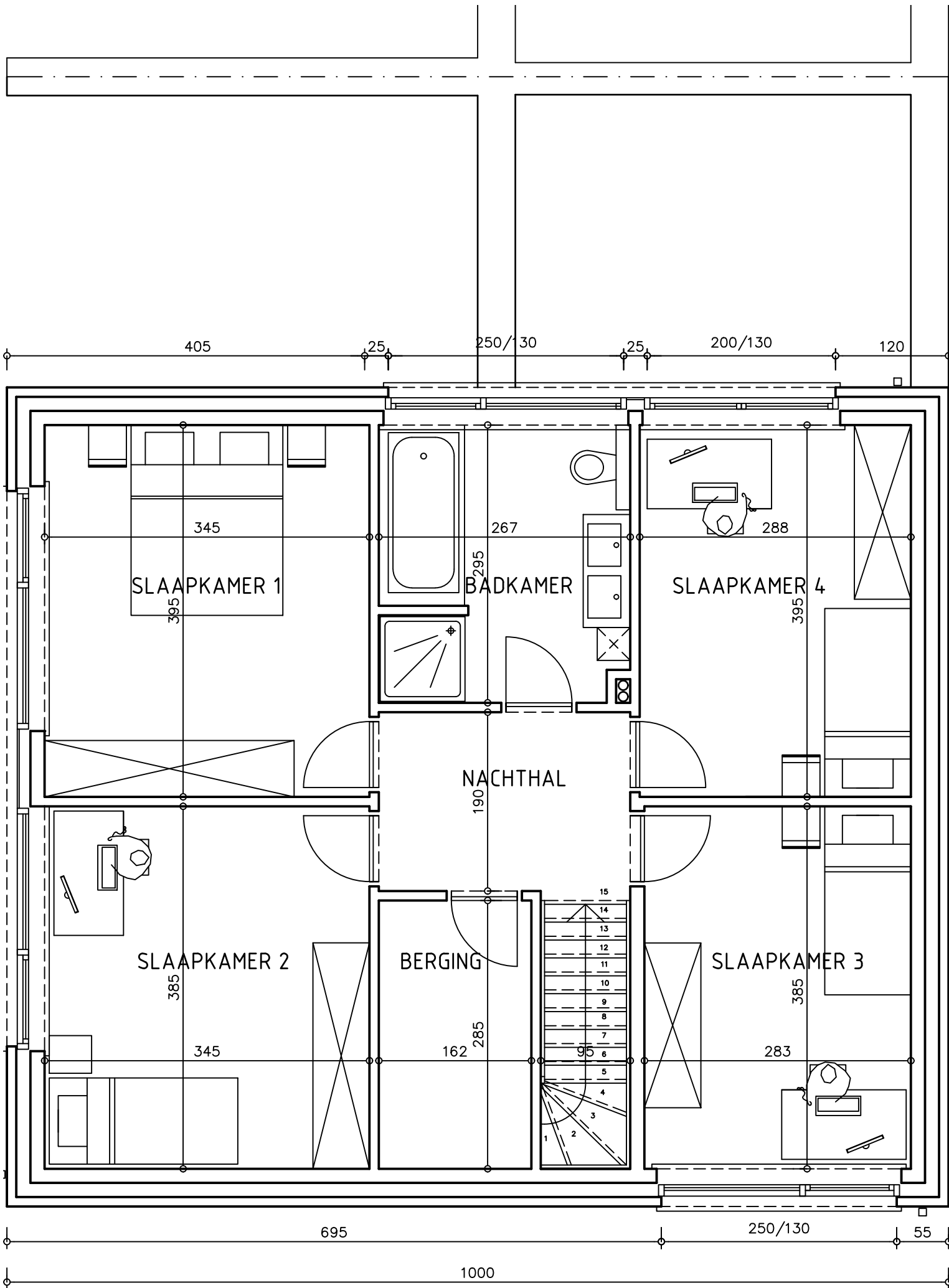
LOT J12 VERDIEPING
